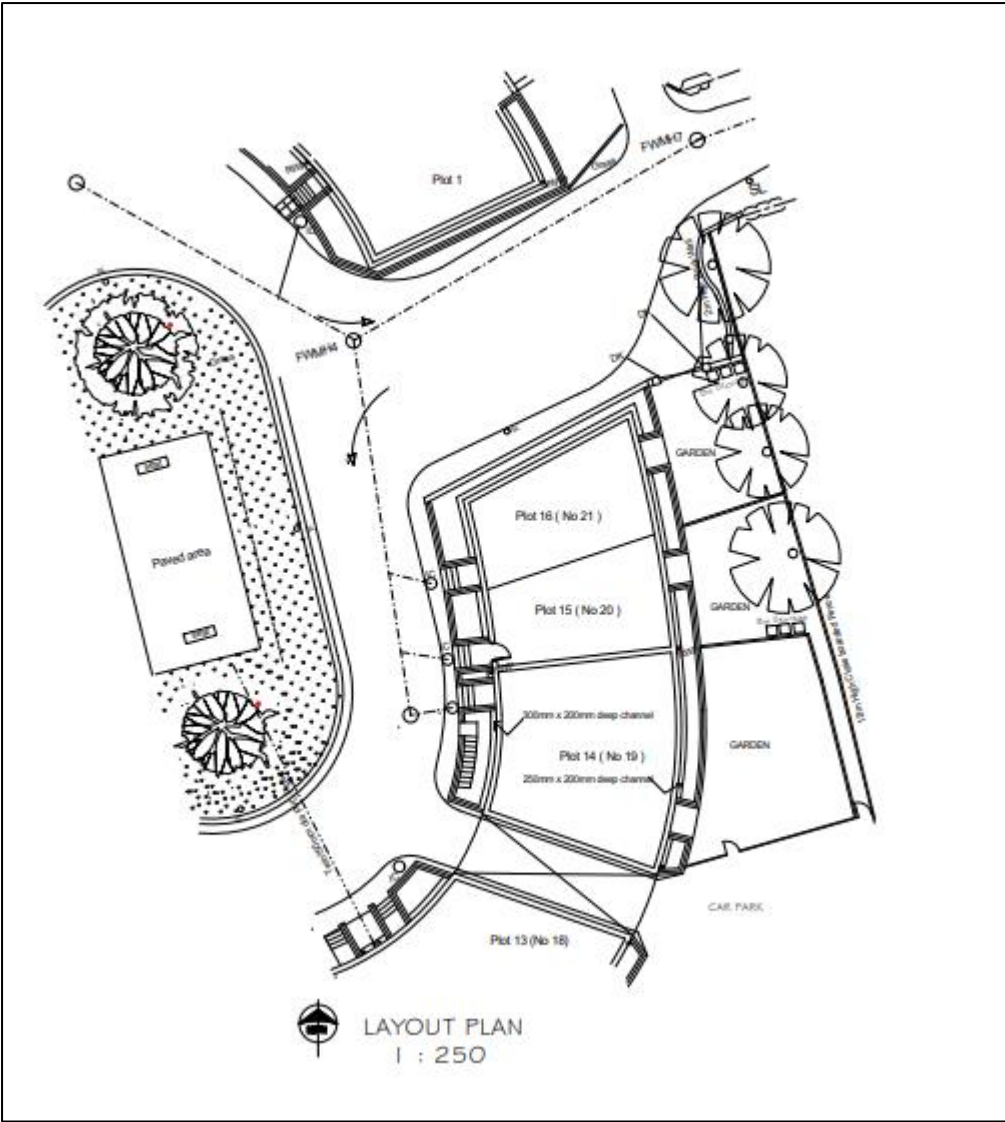
Block Plan
